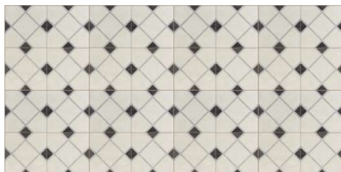
Simulation
